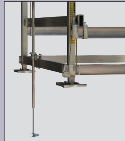
Lift Anchoring System Augers into lake bottom. Works well in soft lake bottoms.
